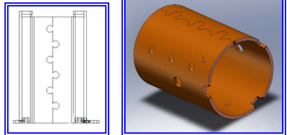
Rolled Formed Fourslide Ring
