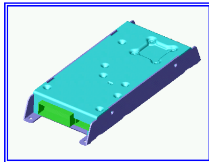
2-Part Stamping
